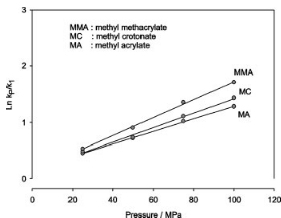
Figure 1. Pressure effect on relative rate constants in the addition of tert -butylamine to methyl acrylates (CH 3 CN, 308.9 K)
